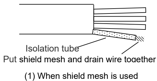
Fig. 4.2 Process shield
