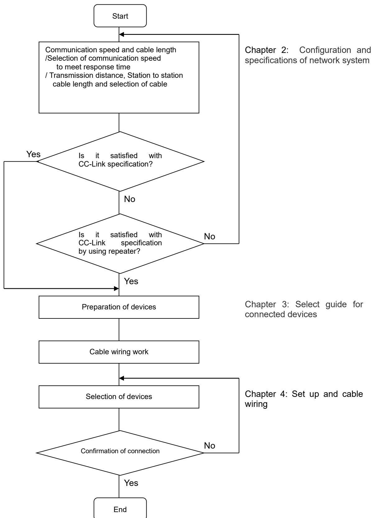
Fig. 1.1 Procedure for cable wiring of CC-Link network system
