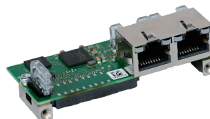
Built-in Module comX 90
