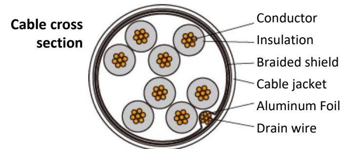
SF/UTP (Double shield structure)
